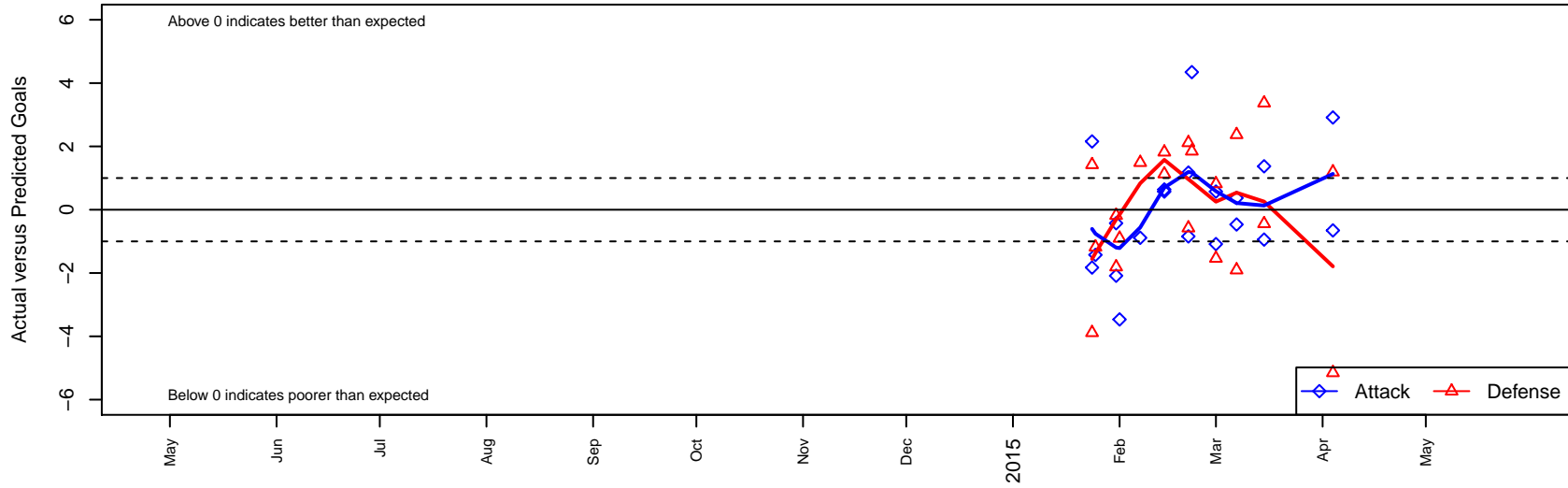
Pelada FA Mariposas B98 Dots are actual minus expected GF (blue circles) and GA (red triangles). Blue line is smoothed change in attack strength. Red is smoothed change in defense strength.
